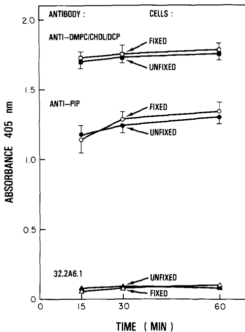
Fig. 2. Binding of anti-DMPC/CHOL/DCP and anti-PIP to macrophage cultures as determined by ELISA. 5 \cdot 10^4 para-formaldehyde-fixed or viable macrophages were incubated at 20^\circ\text{C} for the indicated times with a 100-fold dilution of either anti-DMPC/CHOL/DCP, anti-PIP, or 32.2A6.1 and ELISA was performed. Data shown represent means \pm S.D. of triplicate cultures.
