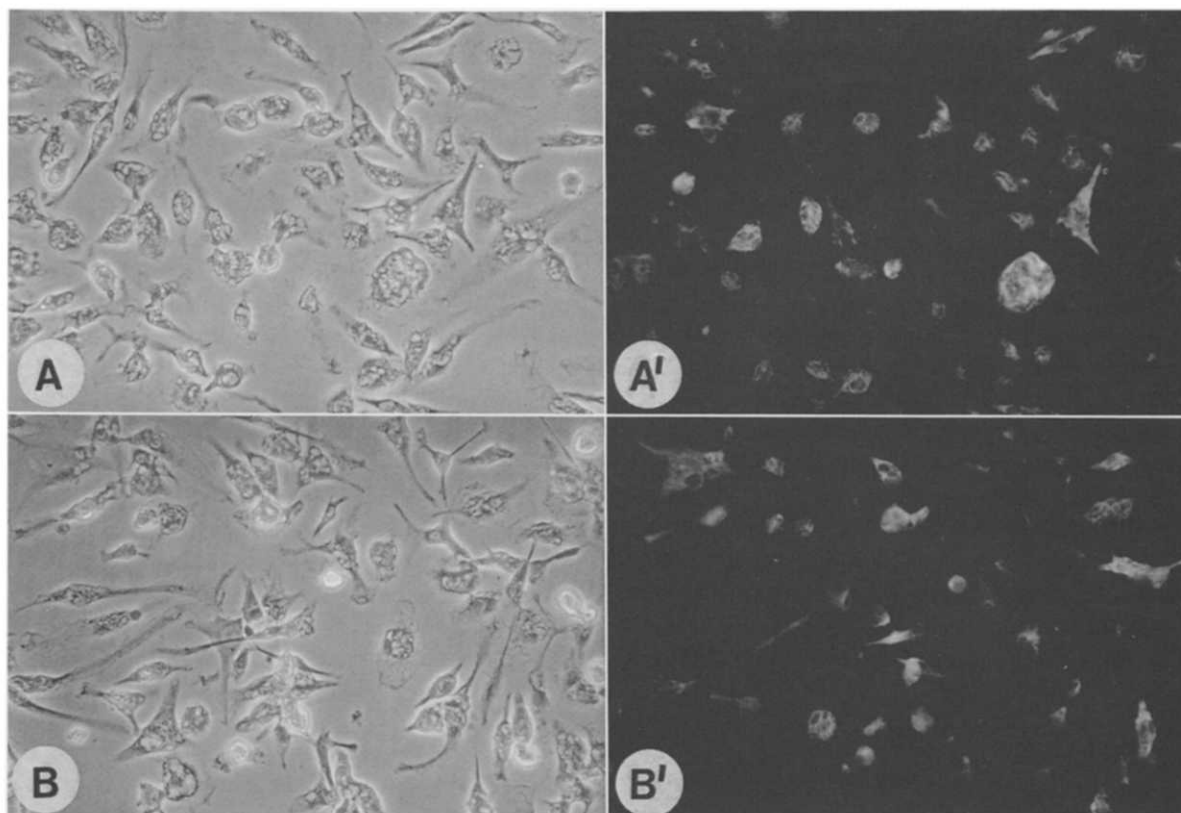
Fig. 1. Indirect immunofluorescence detection of cell-surface bound anti-DMPC/CHOL/DCP and anti-PIP. Macrophage cultures were processed as described in Materials and Methods. (A) Phase-contrast micrograph of macrophage cultures incubated with anti-DMPC/CHOL/DCP; (A') immunofluorescence micrograph of field under (A); (B) phase-contrast micrograph of macrophage cultures incubated with anti-PIP; (B'), immunofluorescence micrograph of field under (B) ( \times 350 ).
