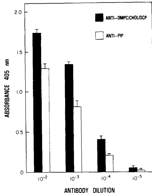
Fig. 3. Titration of the cellular immunoreactivity of anti-DMPC/CHOL/DCP of anti-PIP. 5 \cdot 10^4 macrophages were incubated at 20^\circ\text{C} for 30 min with the indicated dilutions of ascites fluid and ELISA was performed. Data shown represent means \pm S.D. of triplicate cultures.
